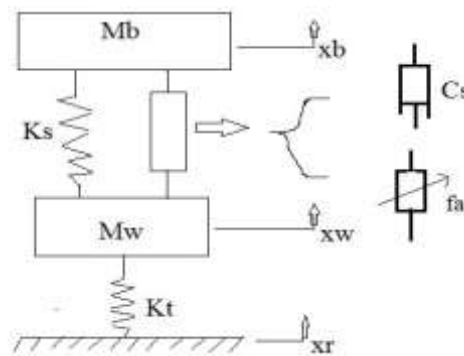
Fig 2:- Passive Suspension System
