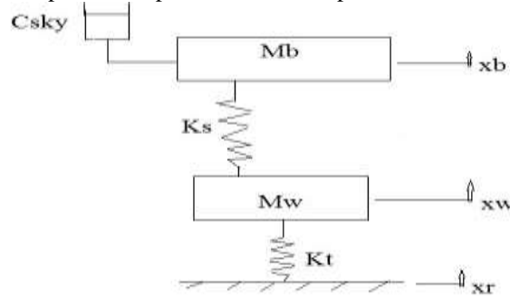
Fig 3:- Skyhook Damper Configuration
